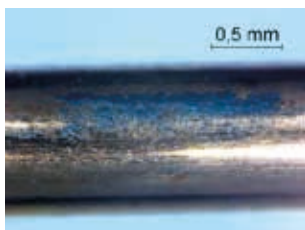
Photo 28: an approximate 15 to 20 µm thick graphite layer on the wire surface. Wire taken out of the graphite filled spiral feed tube after the welding test Item 27 b).
