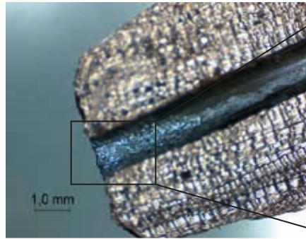
Photo 11: Bisected contact point after a 20 minute welding test with wire as shown in photo 7
